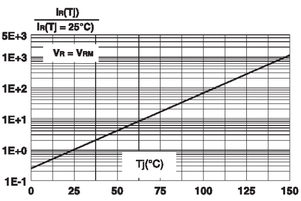
Fig. 7 : Relative variation of leakage current versus junction temperature.
